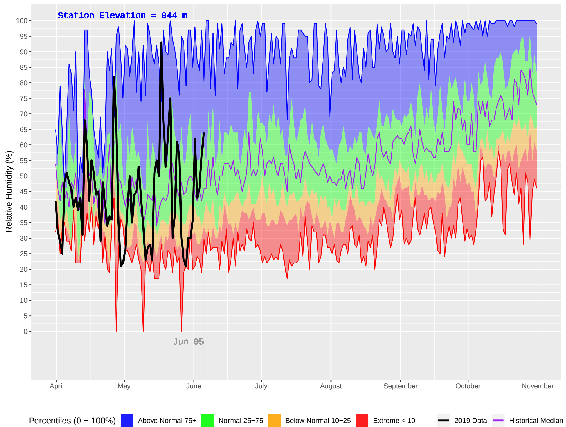
GANOKWA (182) : Historical (1993–2018) and Current (2019) Daily Relative Humidity
