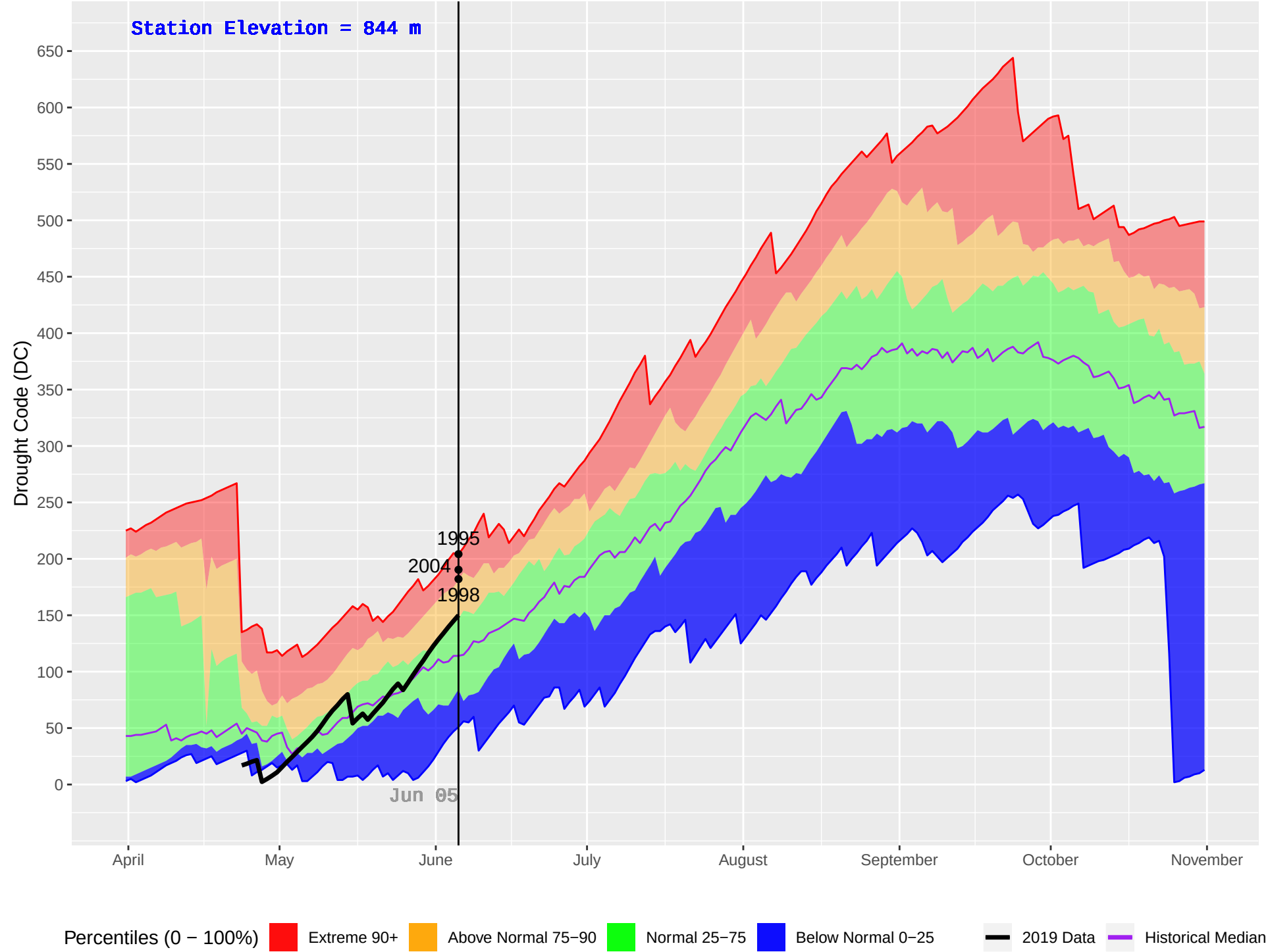
GANOKWA (182) : Historical (1993–2018) and Current (2019) Daily Drought Code (DC)
