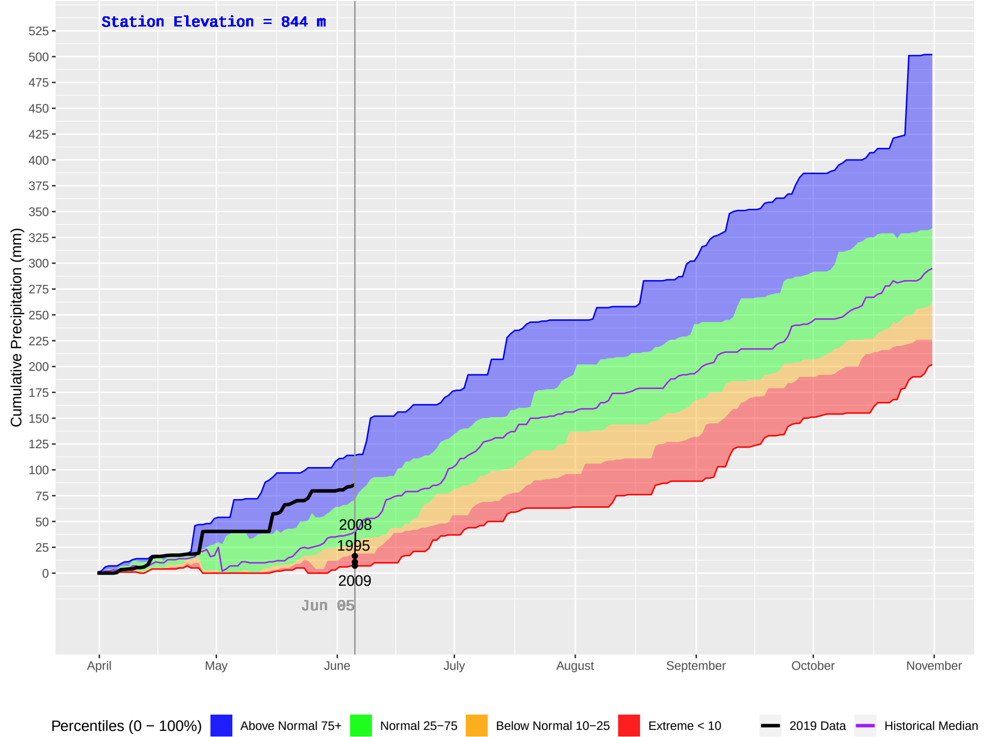
GANOKWA (182) : Historical (1993–2018), Current (2019) Daily Cumulative Precipitation
