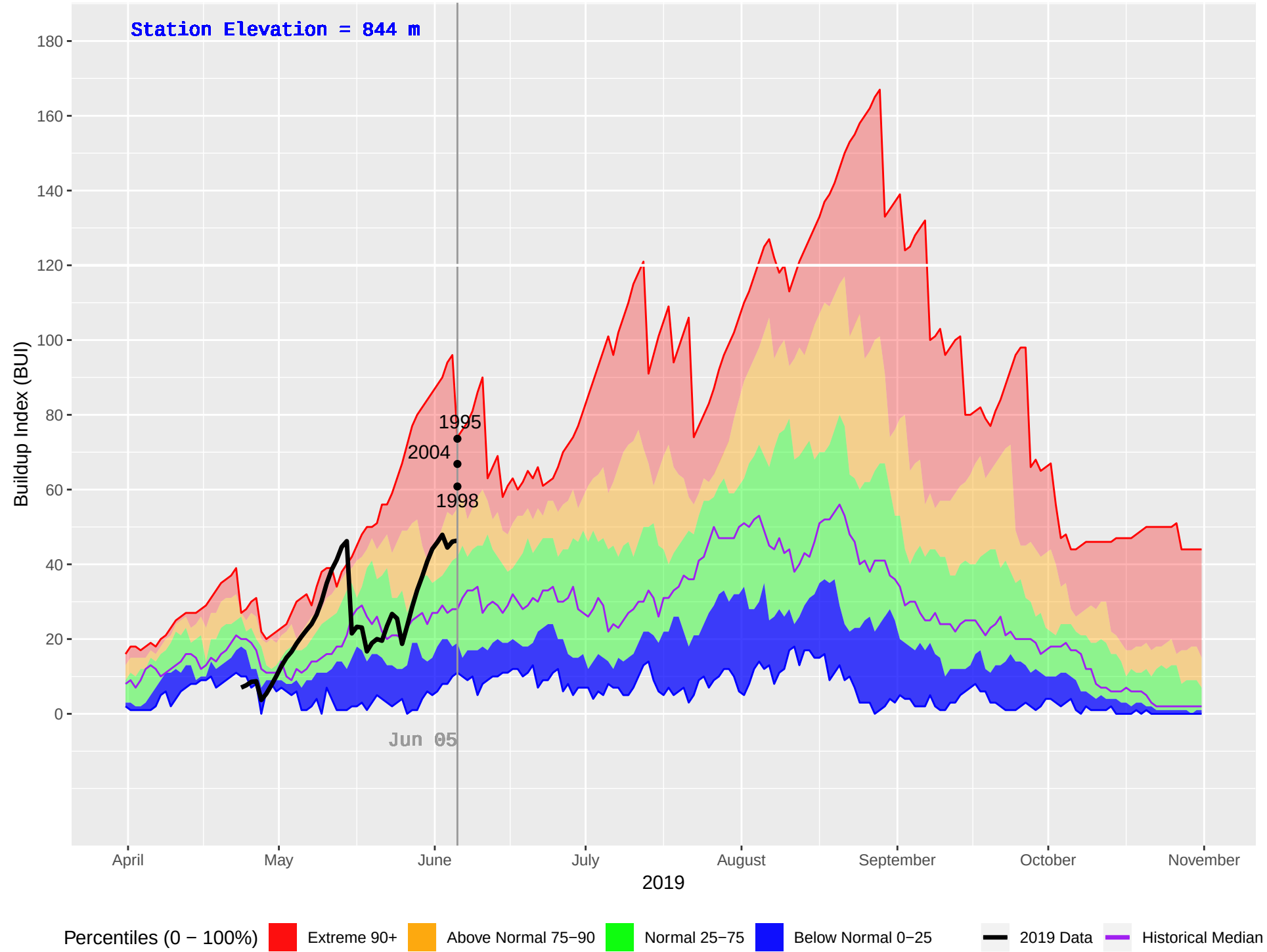
GANOKWA (182) : Historical (1993–2018), Current (2019) Daily Buildup Index (BUI)
