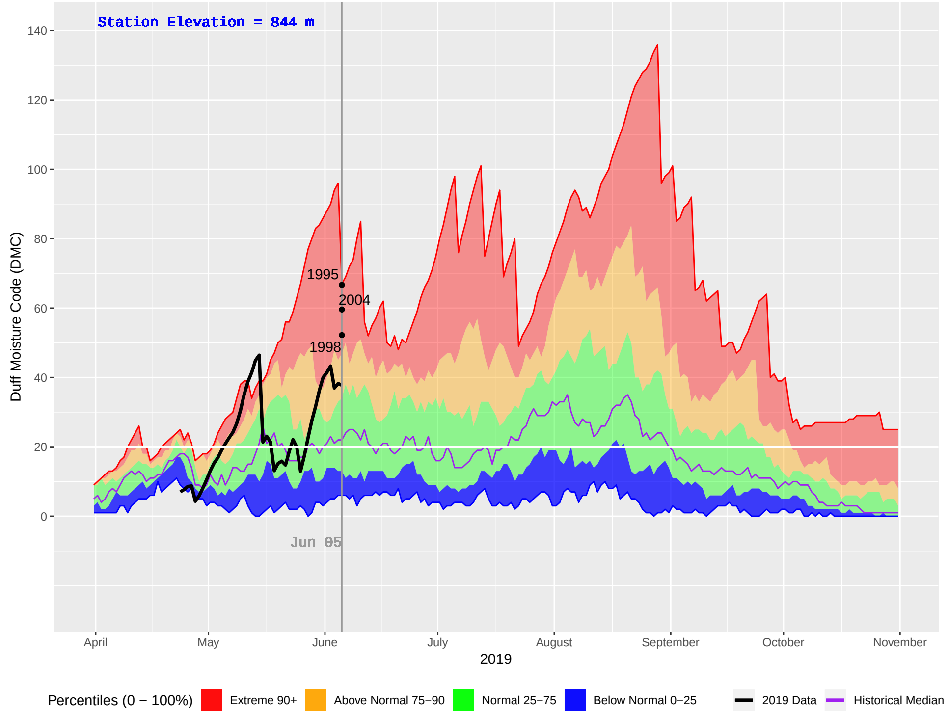
GANOKWA (182) : Historical (1993–2018), Current (2019) Daily Duff Moisture Code (DMC)
