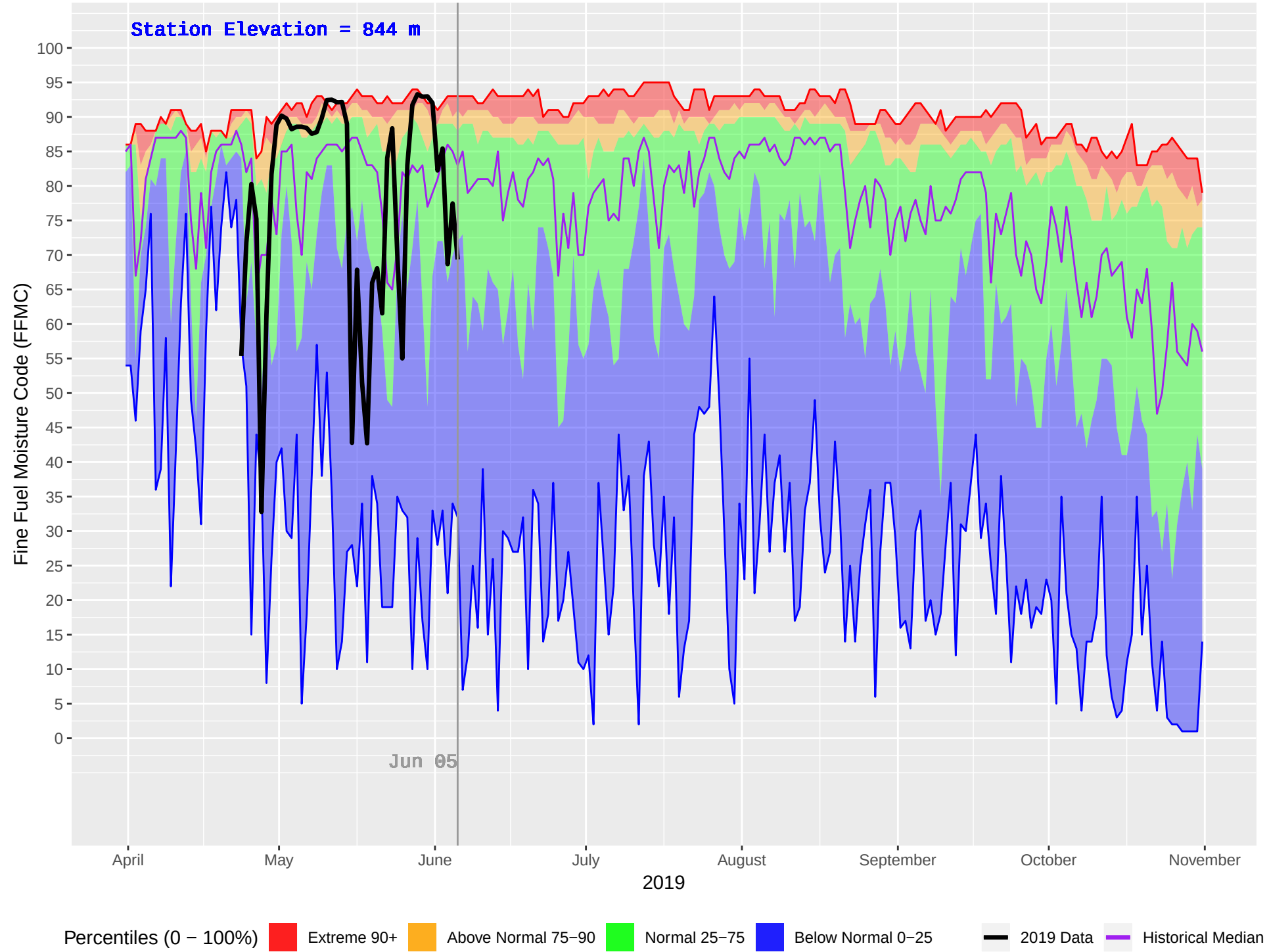
GANOKWA (182) : Historical (1993–2018) and Current (2019) Daily Fine Fuel Moisture Code (FFMC)
